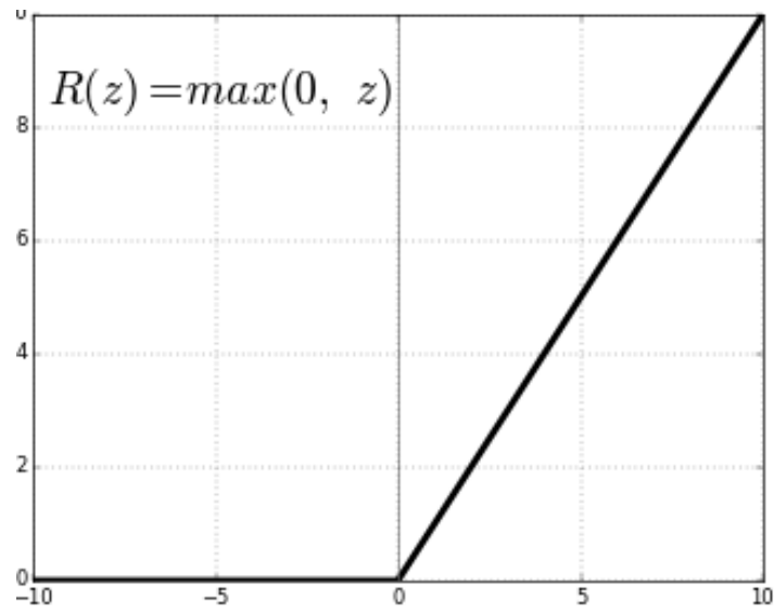
Gambar 5.6 : Rectified Linear
